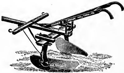
THE SHOVEL POTATO HOE
